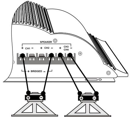
CSA200.3 BRIDGED SPEAKER CONNECTIONS
