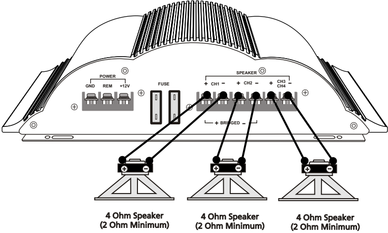
CSA200.3 SPEAKER CONNECTIONS
